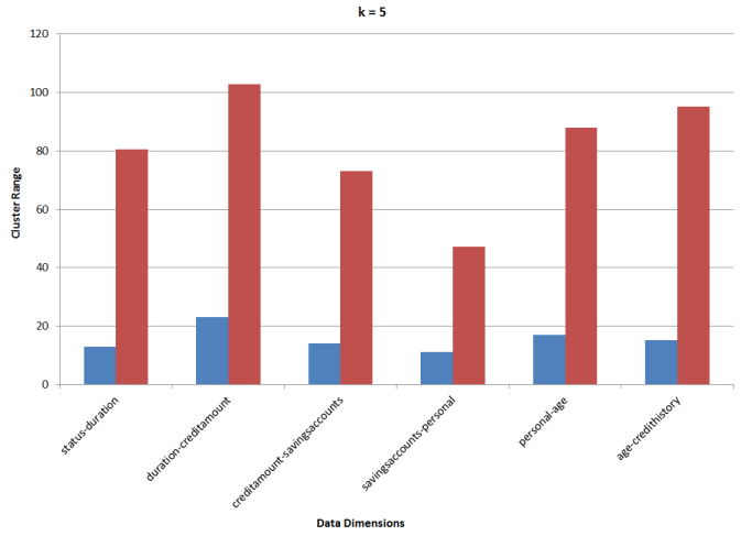
Fig. 10. Multi-dimensional clustering (red bars), as opposed to axis-pairwise clustering (blue bars), leads to high cluster ranges that cause occlusion as shown in Figure 2.
