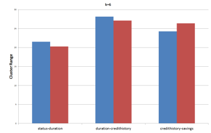
(c) Cluster ranges for seeding with k = 6
