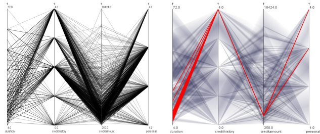
(b) Patterns between credithistory , creditamount and personal
