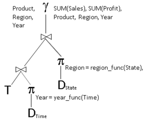
Figure 3. Query structure for the visualization from Fig. 1 after expanding compressed columns to joins and pushing down calculations.
