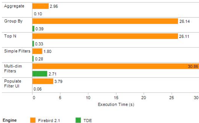
Figure 4. Execution times for selected queries from TPC-H for Firebird and the TDE.
